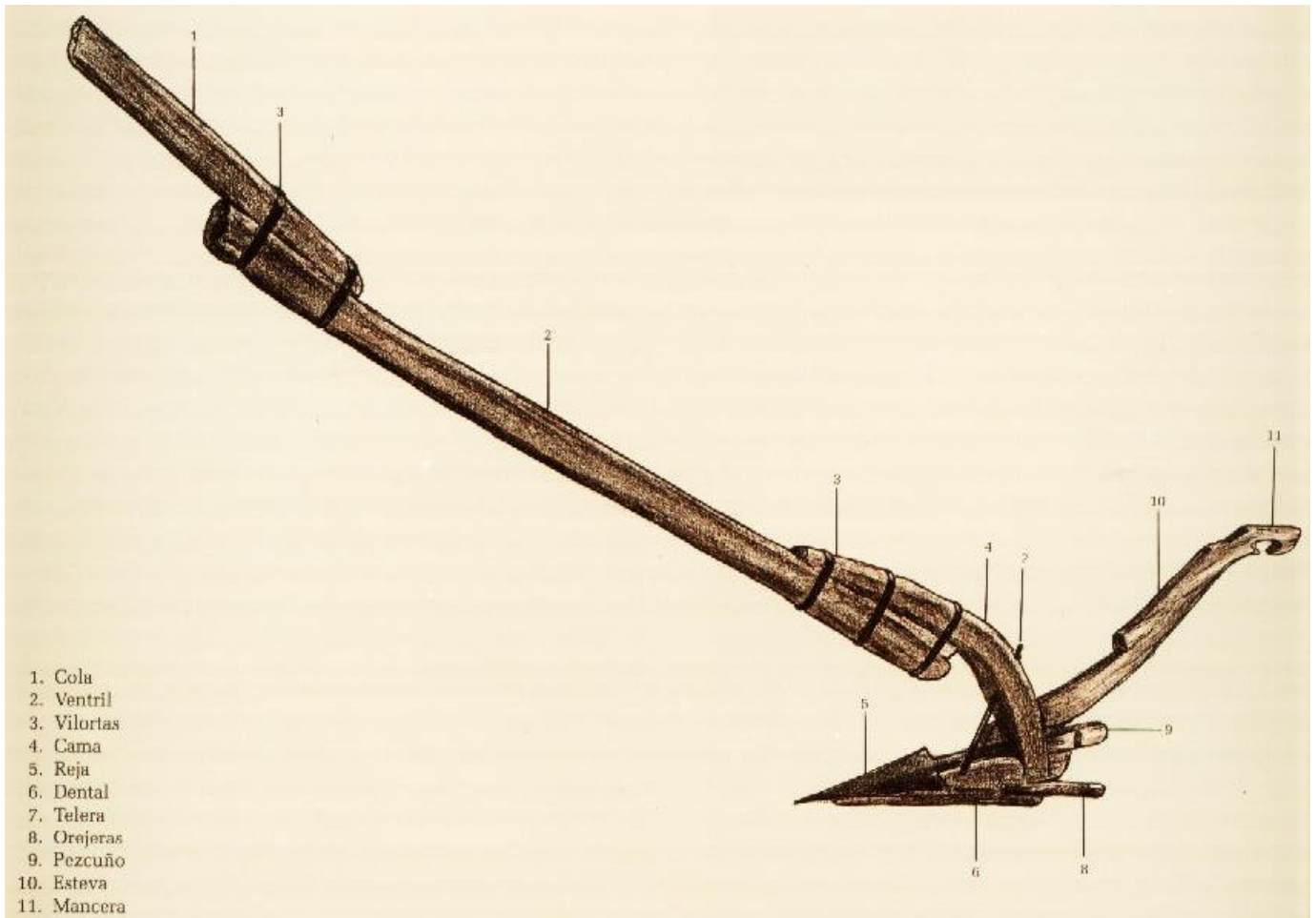
ALADRE – PARTS: 1: Timó- 2: Cameta- 5: Rella- 6: Dental- 8: Orellera- 9: Tinella-10: Esteva
